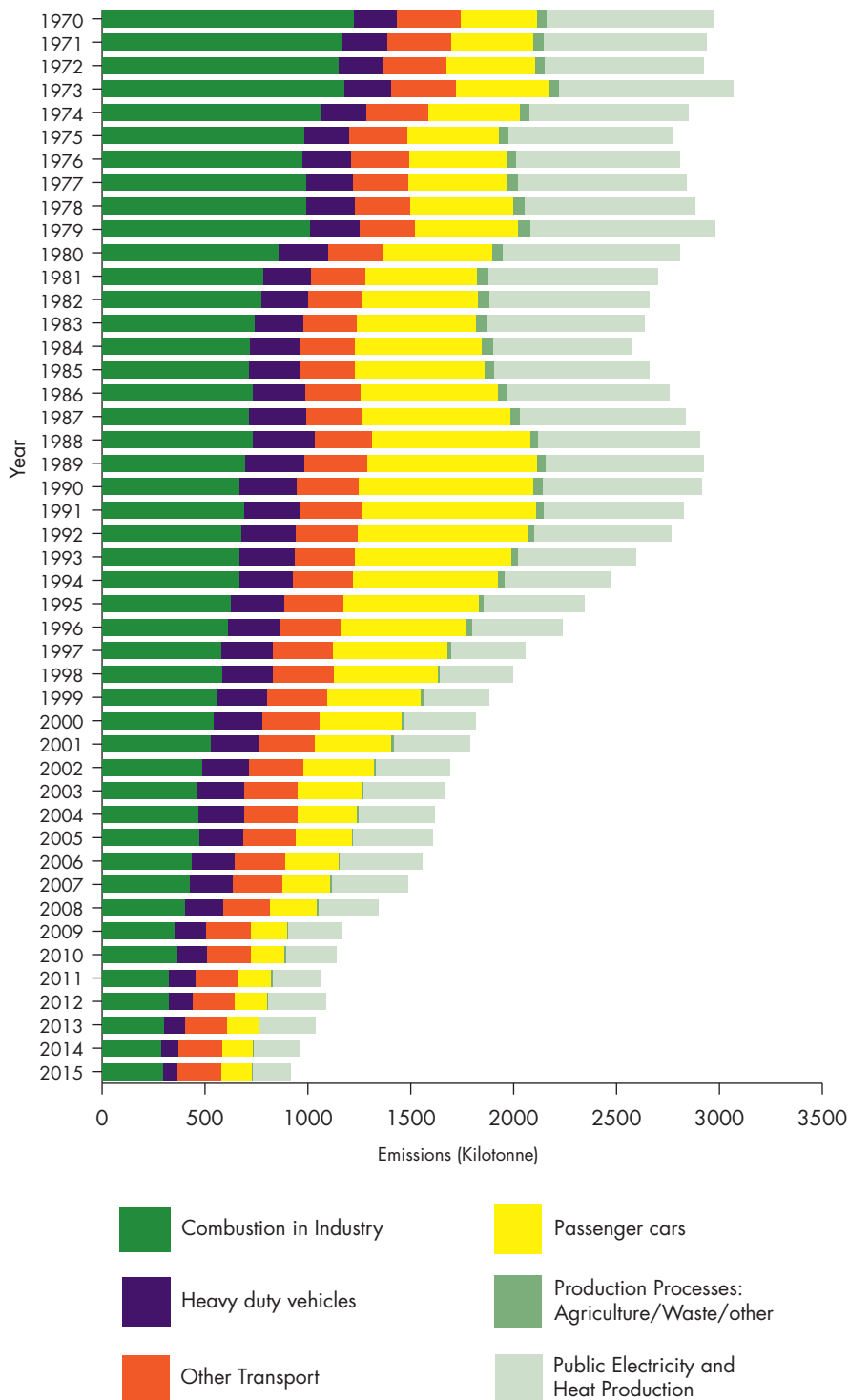
Figure 2: Source of Nitrogen Oxides emissions between 1970 and 2015.
